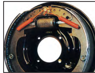
➤ Hydraulic Brakes
